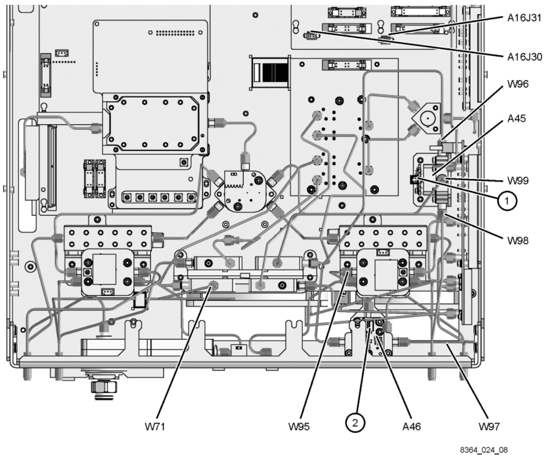
Figure 12 Cable Installation, Analyzers with Options UNL, 014, and 080
